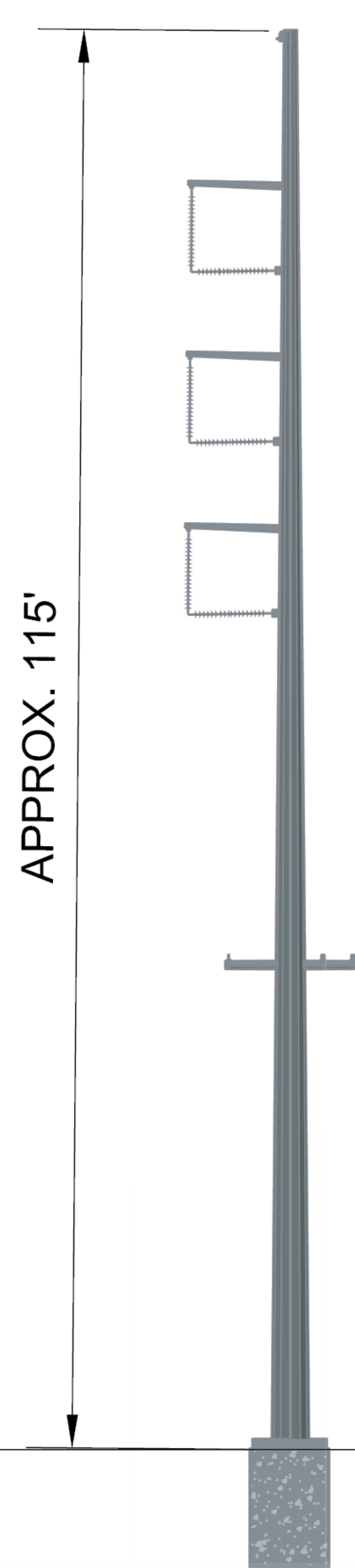
PROPOSED SINGLE CIRCUIT 161kV WITH DISTRIBUTION
