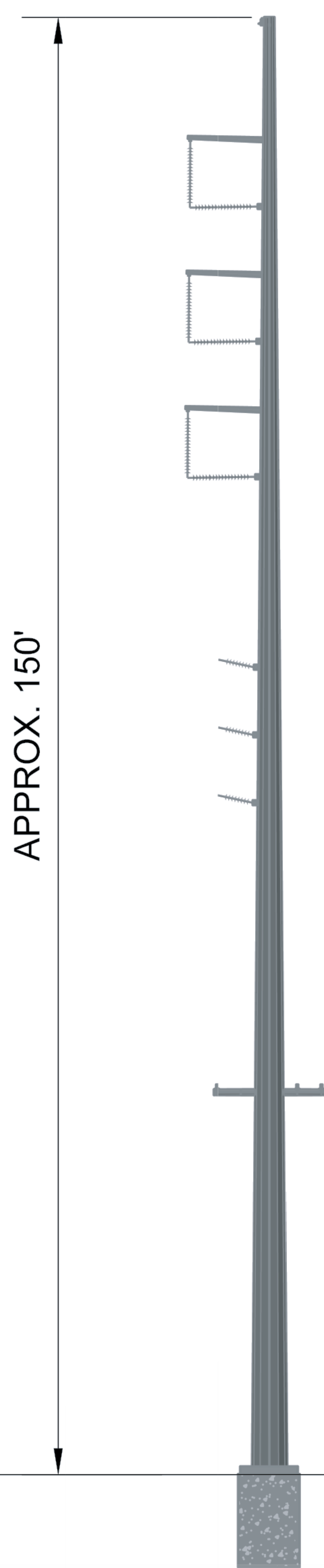
PROPOSED DOUBLE CIRCUIT 161 kV/69kV WITH DISTRIBUTION
