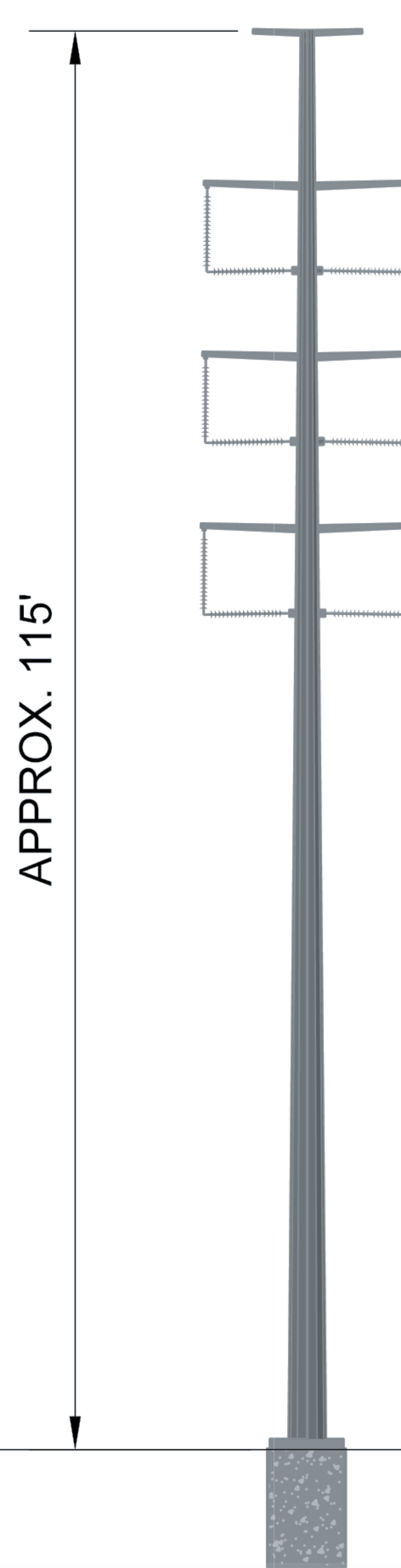
PROPOSED DOUBLE CIRCUIT 161kV
